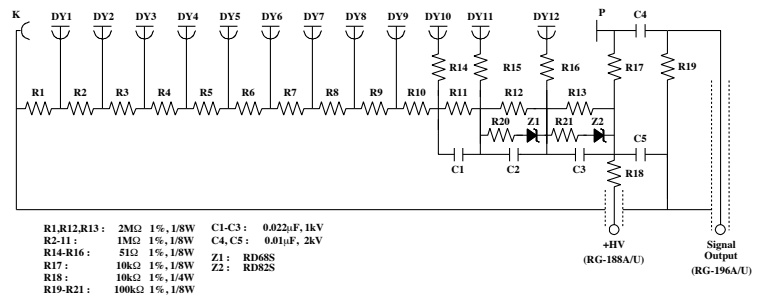
Figure 2.19: Picture of PMT (left) and diagram (right) [73].
