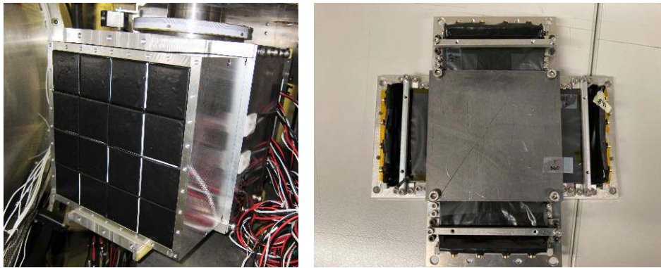
Figure 2.25: BGO crystal (left) + pre-shower timing counter (right) [35, 50].
